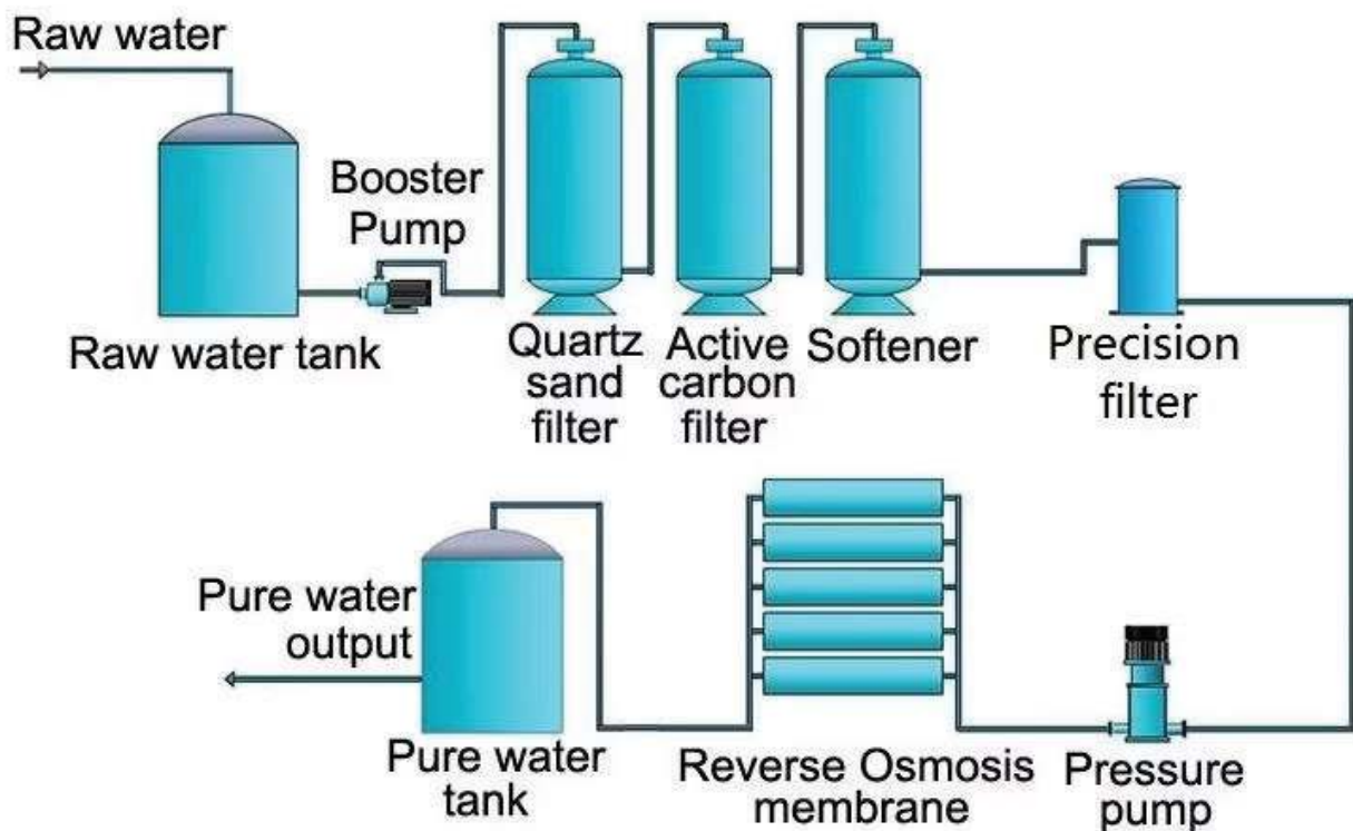
RO Flow Chart
